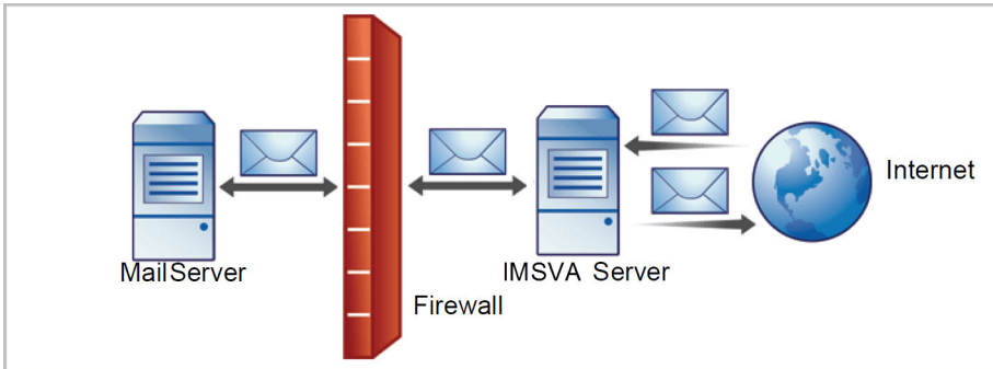
FIGURE 3-6. Installation topology: in front of the firewall
