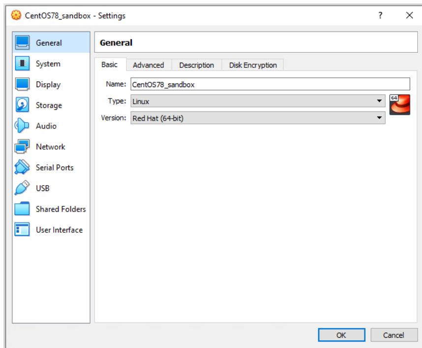
FIGURE 4-10. VirtualBox Settings
